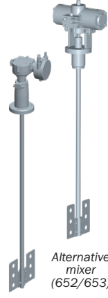
Rotary mixer (652/653)
